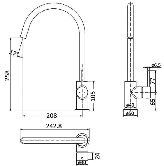
HYB88-101BN - Hali Gooseneck Sink Mixer - Brushed Nickel
